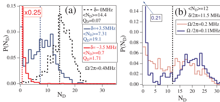
Figure 3. P(N_D) histograms vs N_D , at 20 \mu\text{s} short interaction time in (a) and dashed red line in (b), and a long interaction time blue solid line in (b). In (a) for positive detuning (blue line) the histogram exhibits a bimodal structure; on resonance (black dashed line) it has a single peak, and for negative detuning (red line) \langle N_D \rangle is considerably smaller. In (b) the probabilities histograms show the crossover to the dissipative regime with the counting distribution strongly bimodal at 950 \mu\text{s} interaction time. As the excitation duration is increased, the Rabi frequency is decreased in order maintain \langle N_D \rangle constant.
