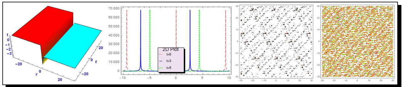
Figure 2. Plot of 3D, 2D, density and contour of (24)
