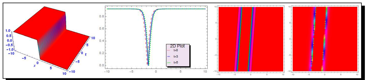
Figure 4. Plot of 3D, 2D, density and contour of (26)
