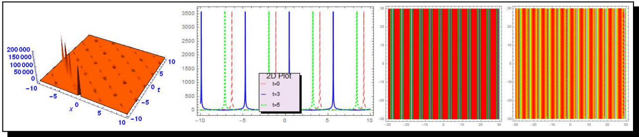
Figure 1. Plot of 3D, 2D, density and contour of (23)
