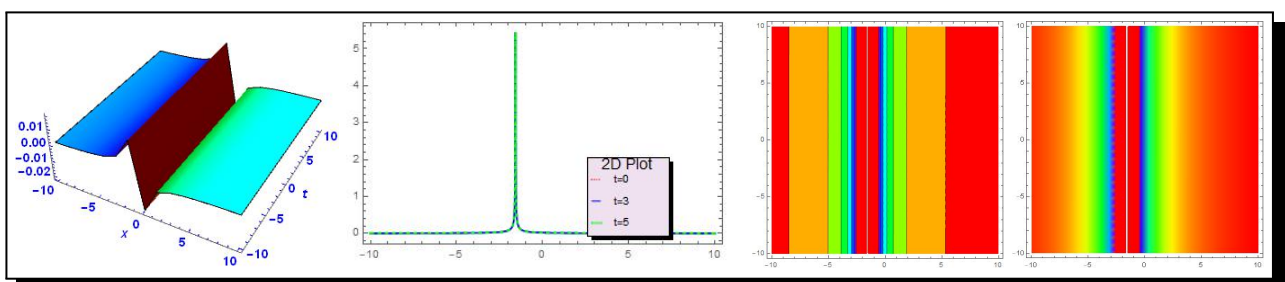
Figure 5. Plot of 3D, 2D, density and contour of (27)
