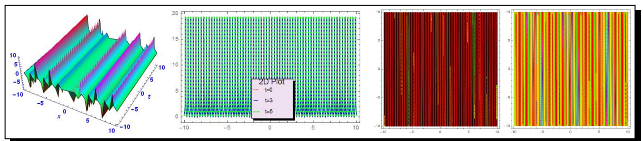
Figure 3. Plot of 3D, 2D, density and contour of (25)
